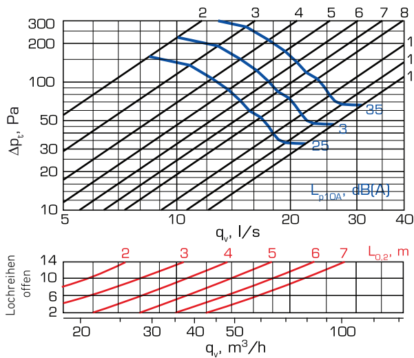
STQA-100
