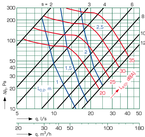
KTI-125
