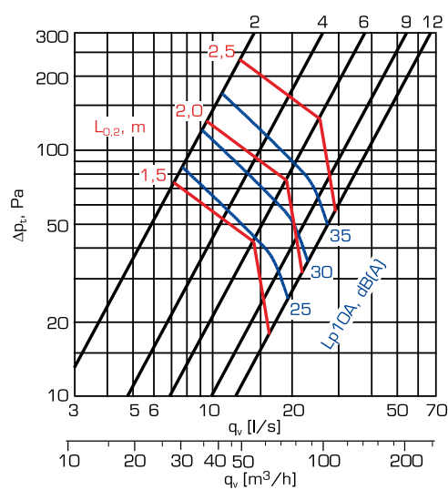
NE-100-C
