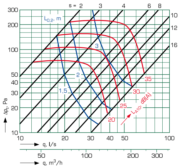
KTI-125
