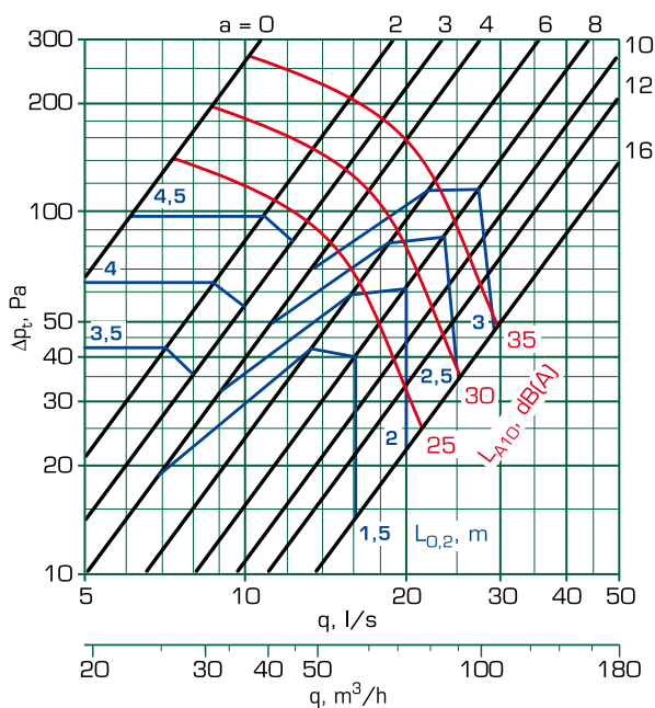
STI-125
