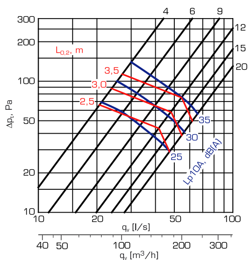
NE-150-C
