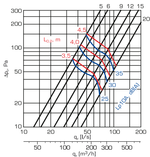
NE-200-C
