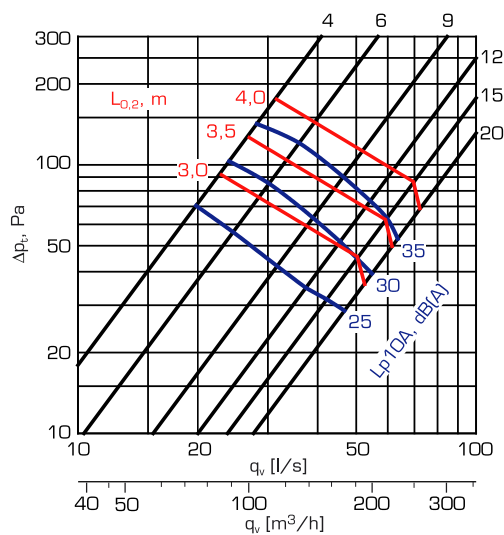
NE-160-C
